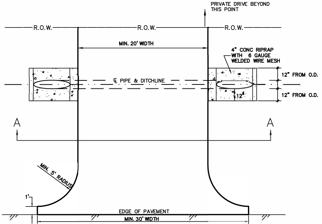
PLAN VIEW
